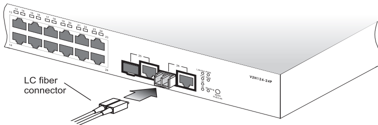
Figure 4-3. Making Fiber Port Connections
